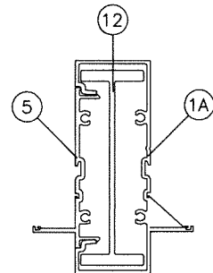
MULLION 'M2A'
