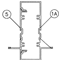
MULLION 'M1A'
